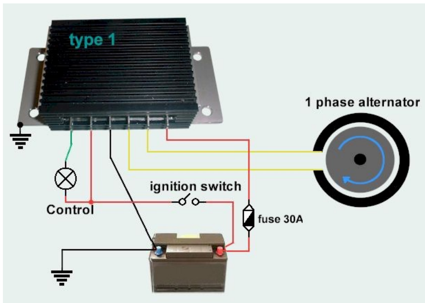
Figure 2 General schematic of how the regulator is connected.
