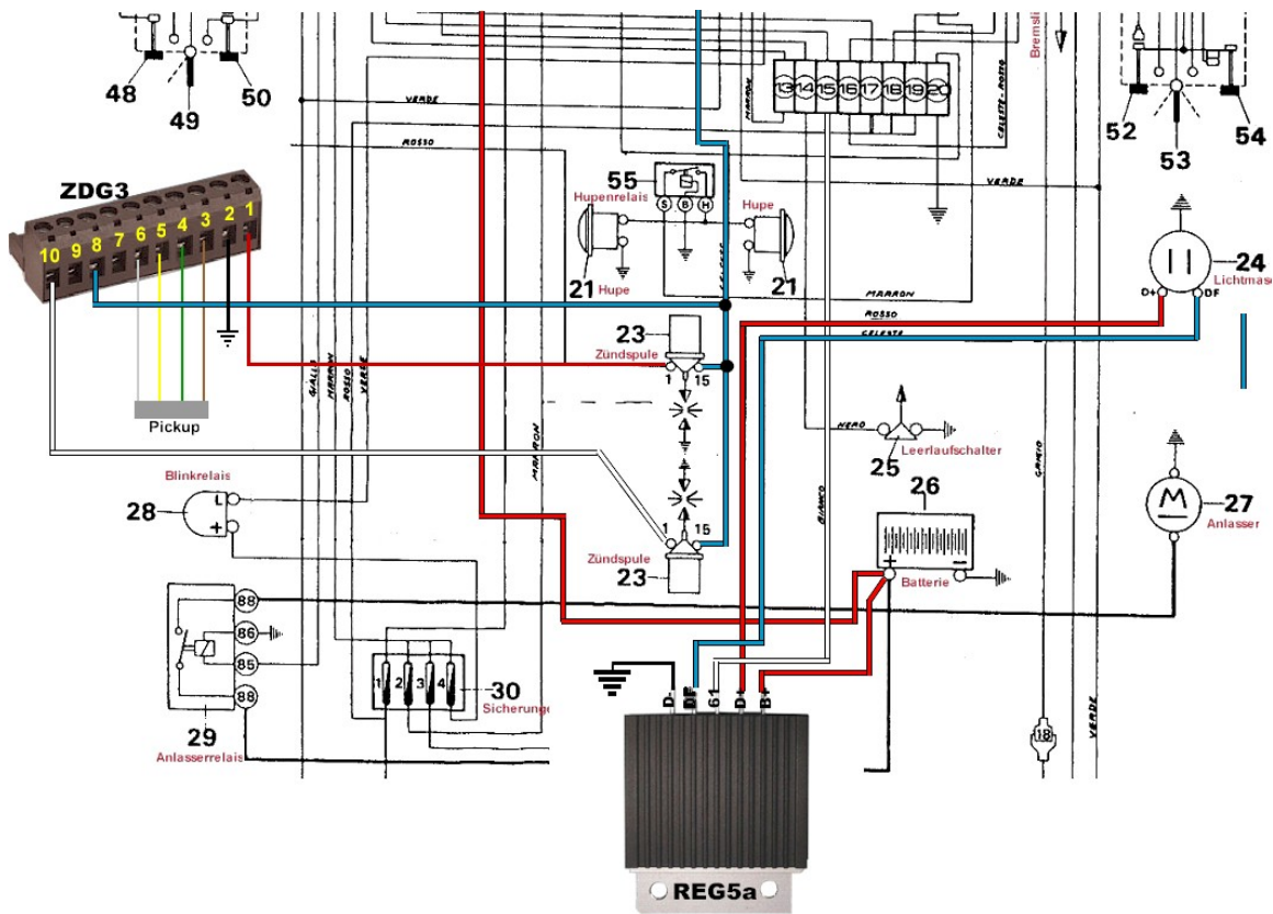
Wiring diagram with regulator
