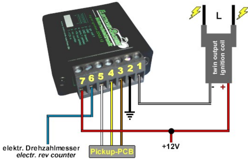
Connection with dual output coil (ZDG 3.12)
