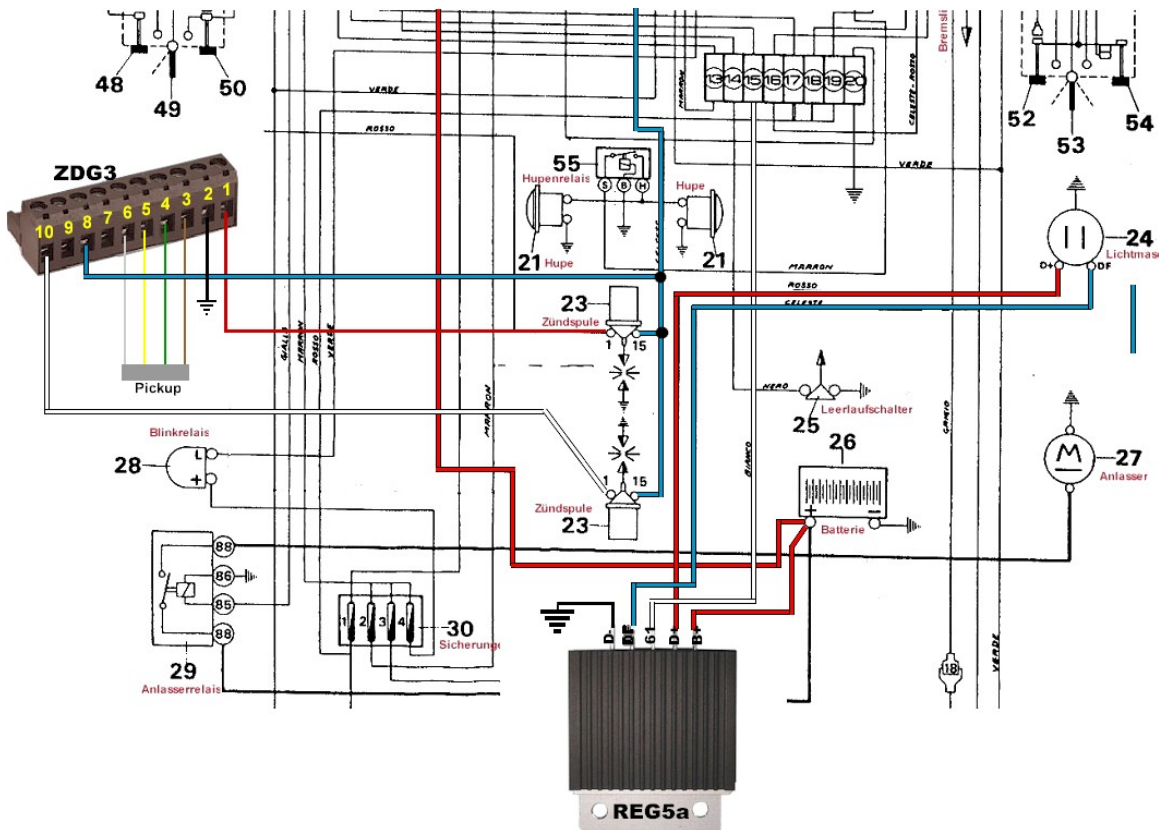
Schematic of the electrical connections with the original two coils (ZDG 3.23)
