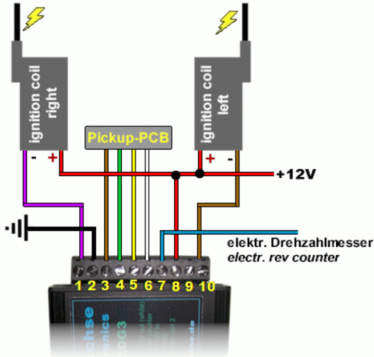
Schematic of the electrical connections with the original two coils (ZDG 3.23)
