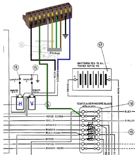
Connection in the original wiring
