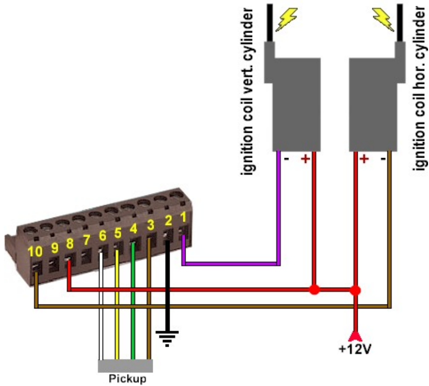
Connection diagram
