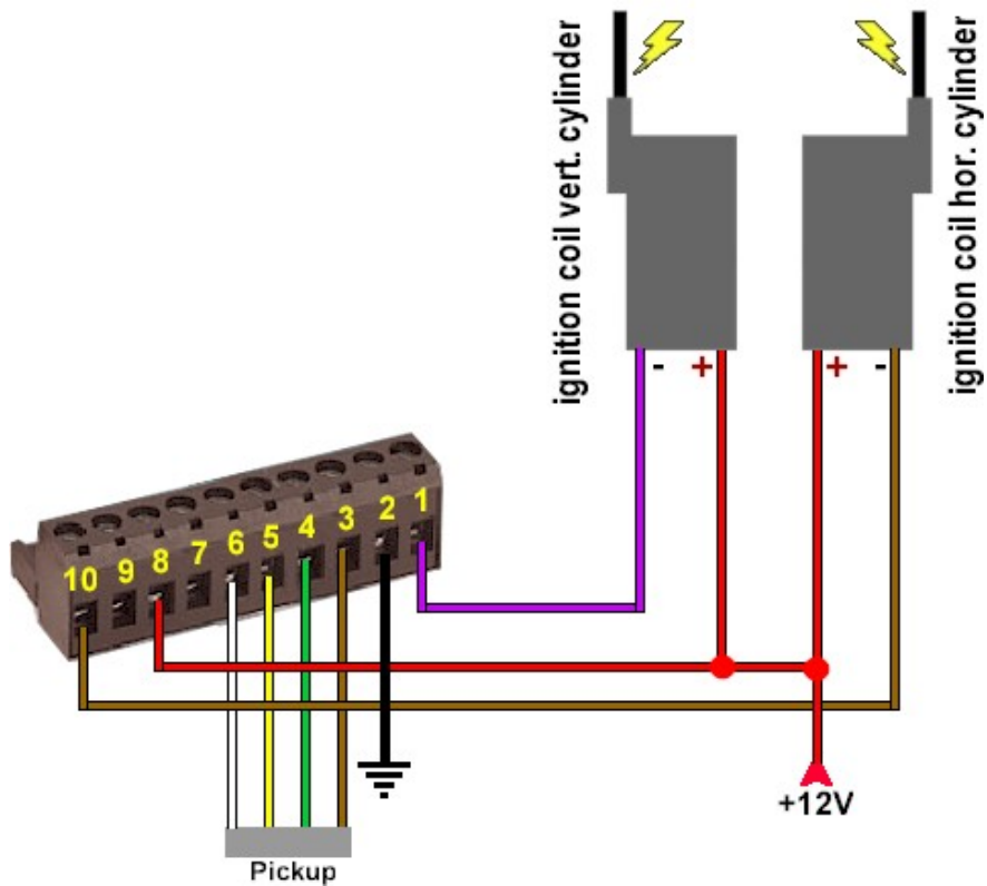
Figure 3 Connection diagram.
