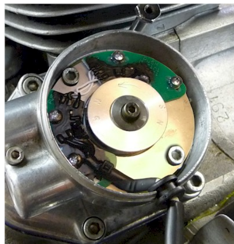
Figure 2.e Final assembly of pickup, driver sleeve and magnet disk.
