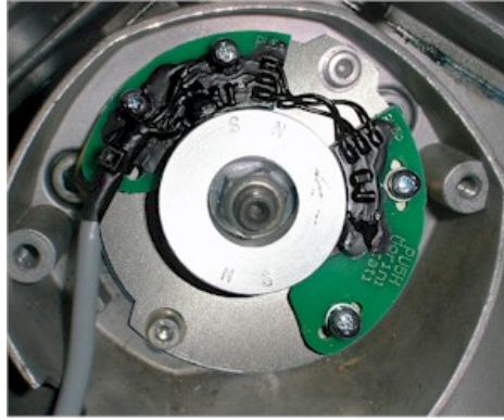
Figure 2.a Assembly of the pickup
