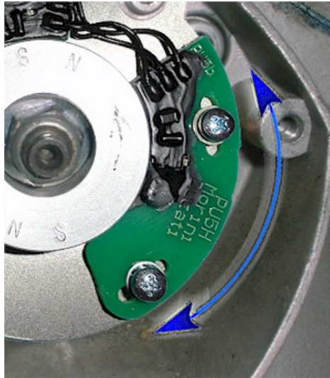
Figure 6.d Fine tuning the advance offset between both cylinders.
