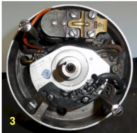
Figure 2.d Mount the new pickup.
