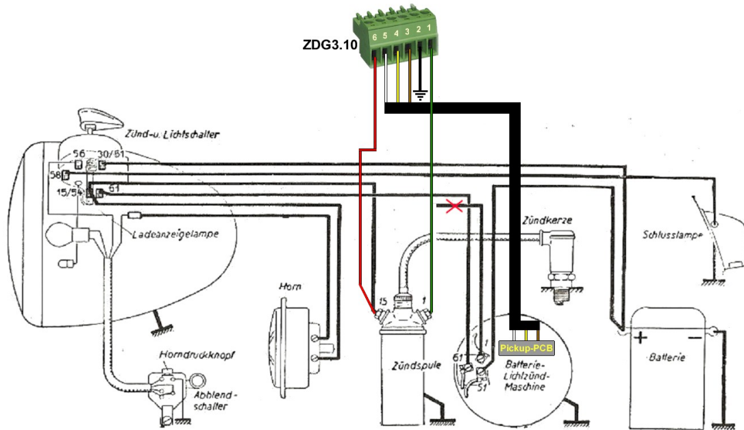
Figure 1 Connection scheme
