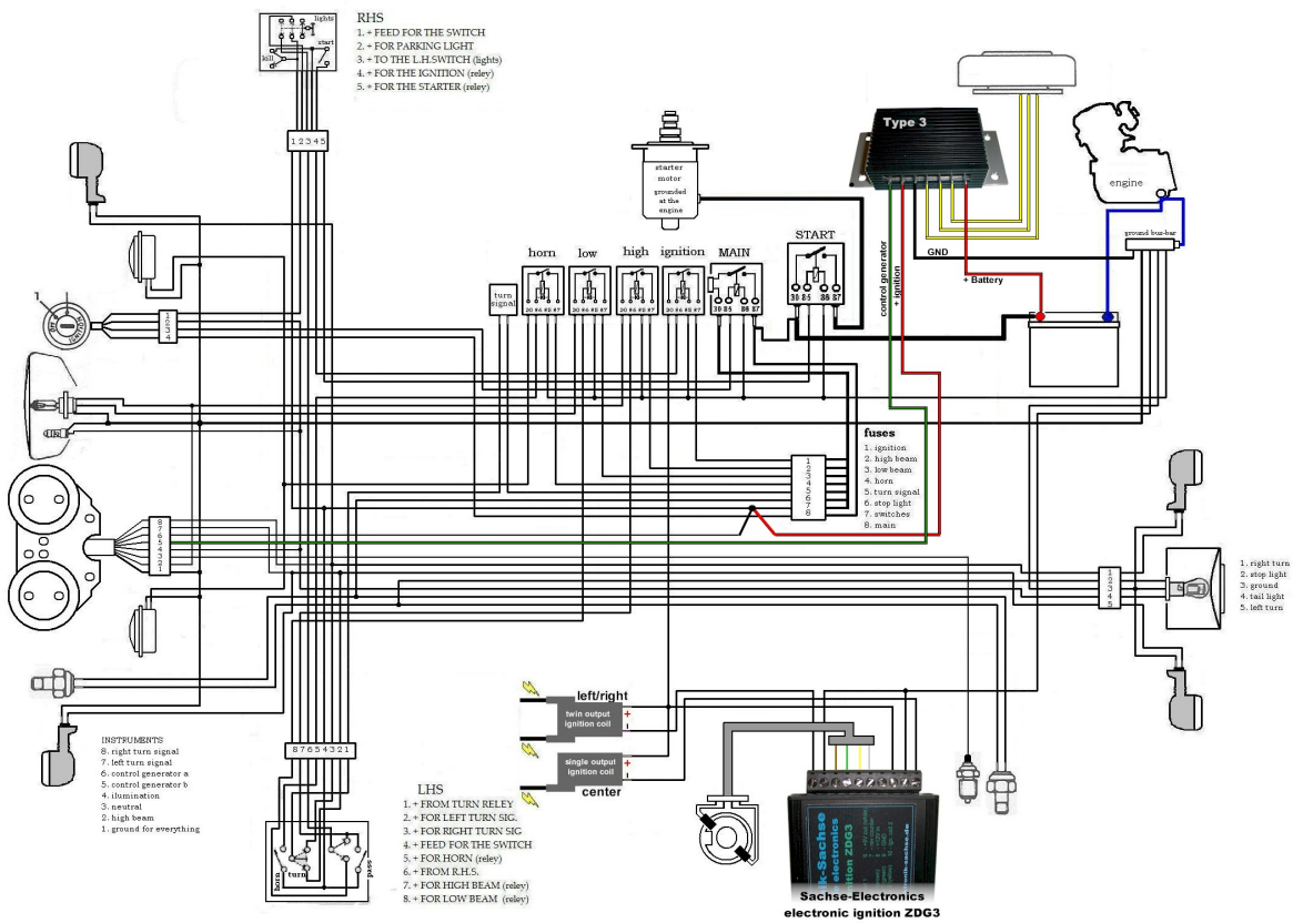
Figure 4 Complete circuit diagram.
