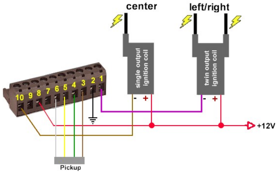
Figure 3 Circuit diagram.
