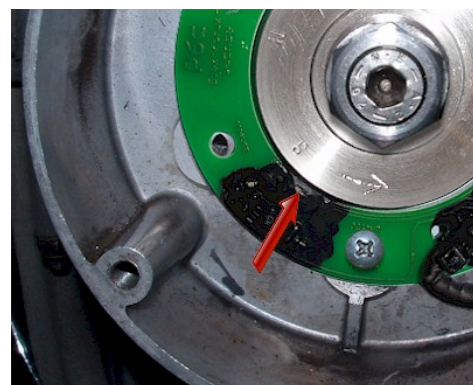
Figure 7 The LED goes off when the piston is on TDC.
