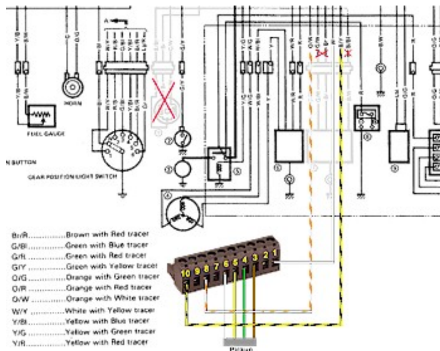
Figure 3 Circuit diagram.
