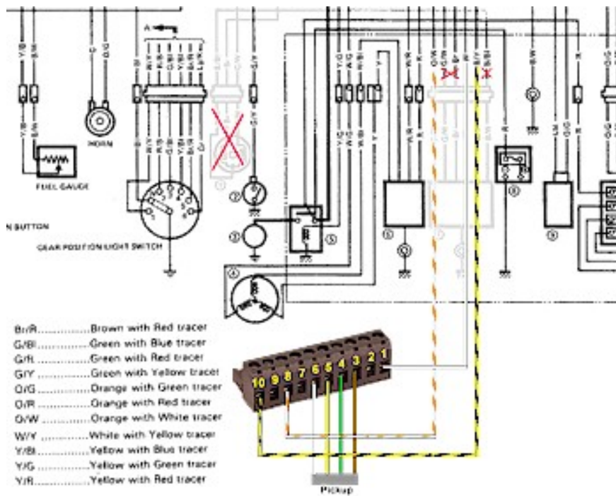
Ignition circuit diagram
