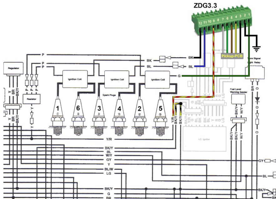
Ignition circuit
