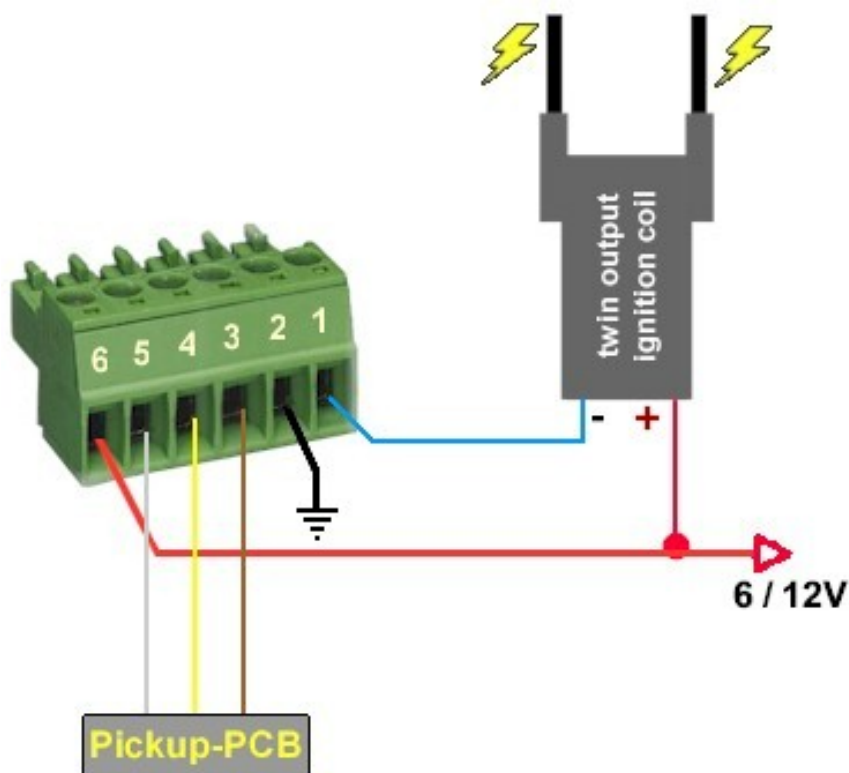
Ignition circuit diagram
