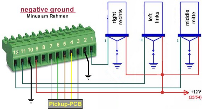
Connection diagram with negative ground
