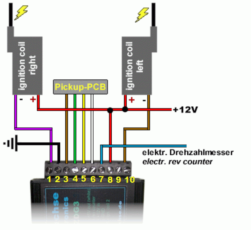
Negative ground – Minus connected to frame
