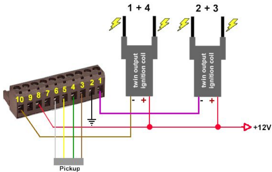
Connection with the wiring diagram
