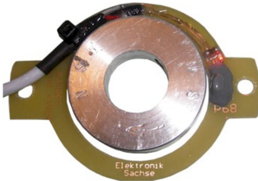
Figure 2 Ensure correct alignment of magnet disk and sensor.
