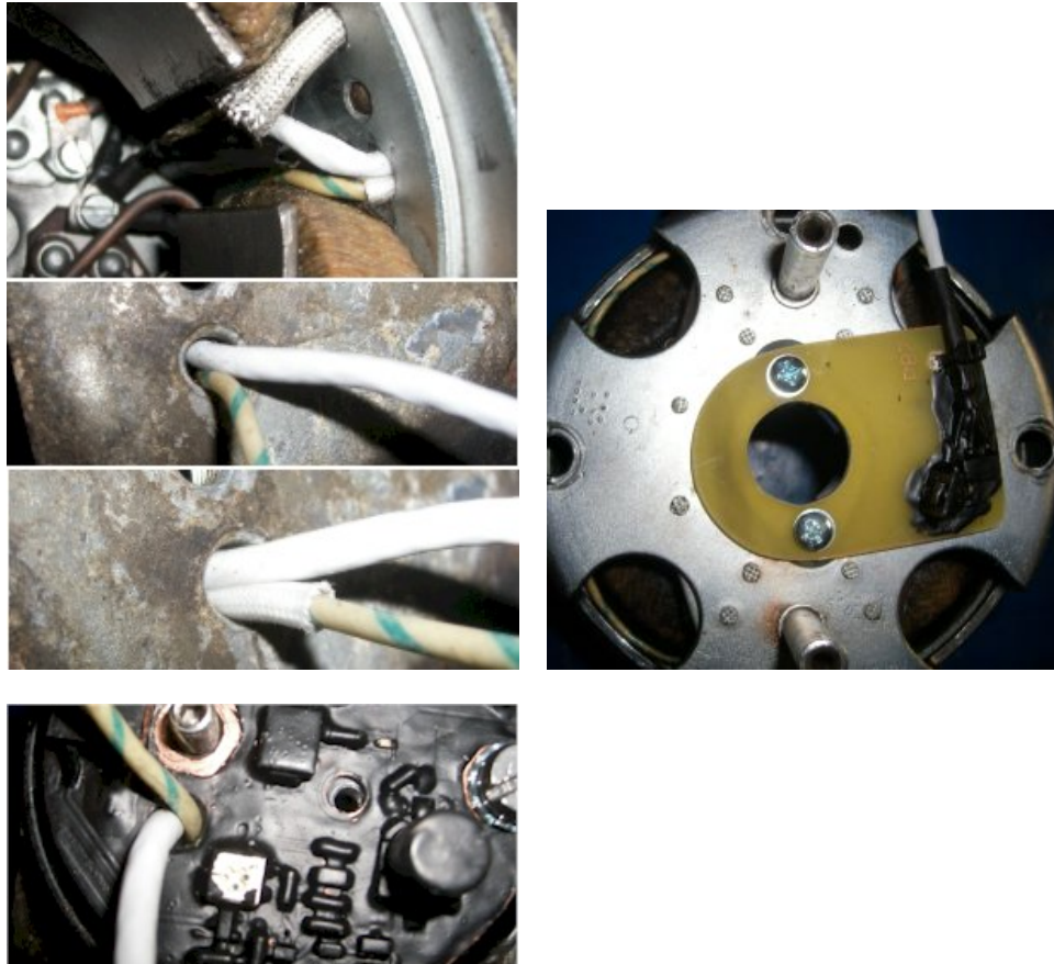
Cable routing through the regulator base plate (in this picture the regulator RegKS is shown)
