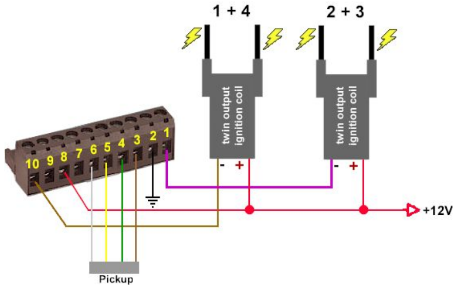
Figure 4 Ignition circuit diagram.
