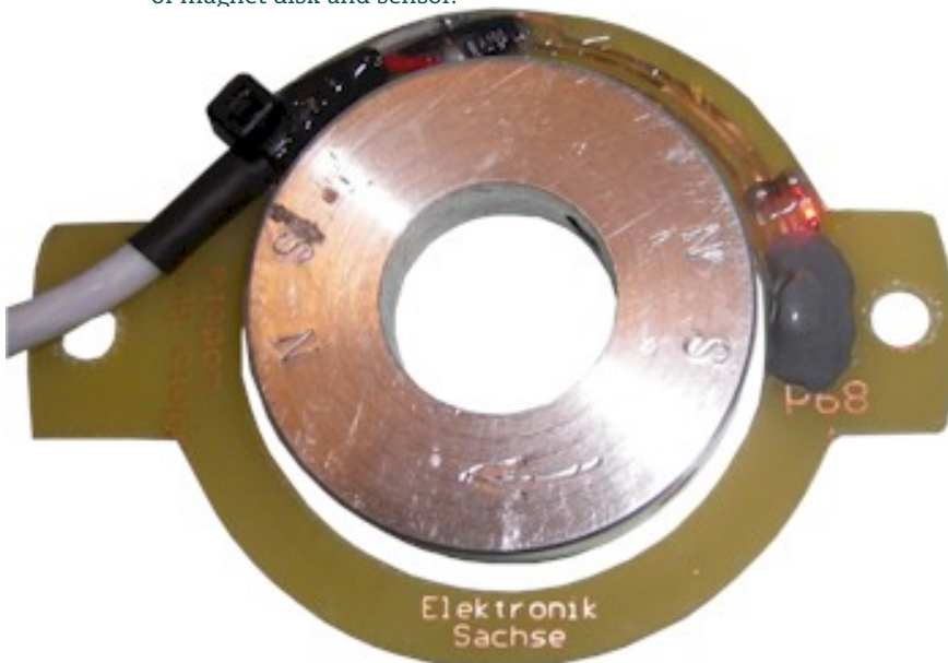
Figure 3 Ensure correct alignment of magnet disk and sensor.
