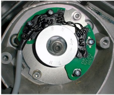
Figure 2 Assembly of the pickup
