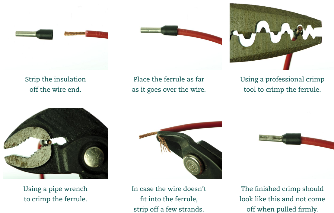
Figure 9 Crimping the wire end ferrules.
