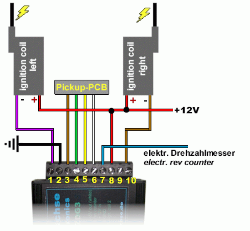
Figure 8 Circuit diagram
