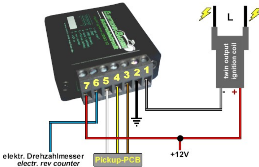
Figure 3 Circuit diagram.
