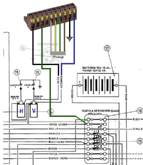
Figure 4 Connection in the original wiring.
