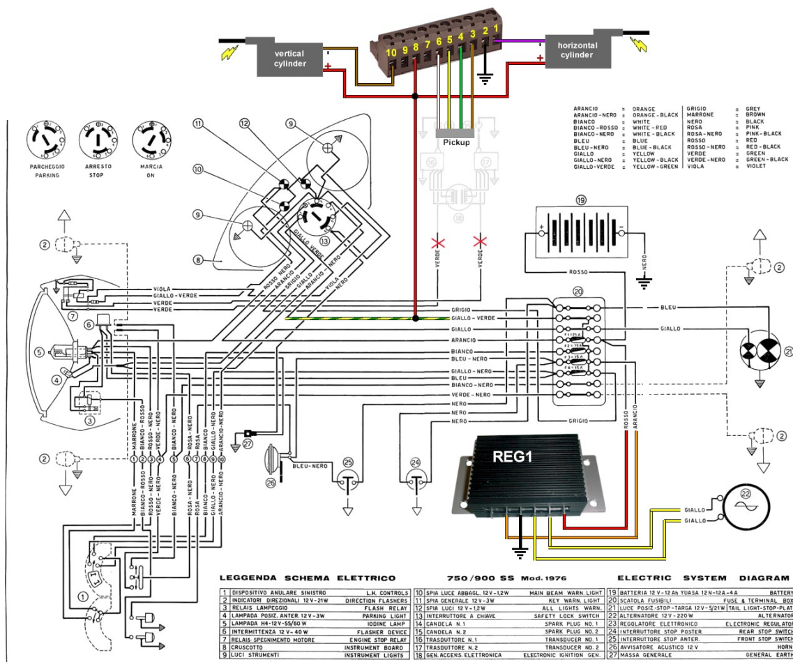
Complete wiring
