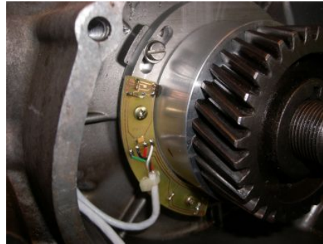
Mounting the new magnet disk on the primary gear.
