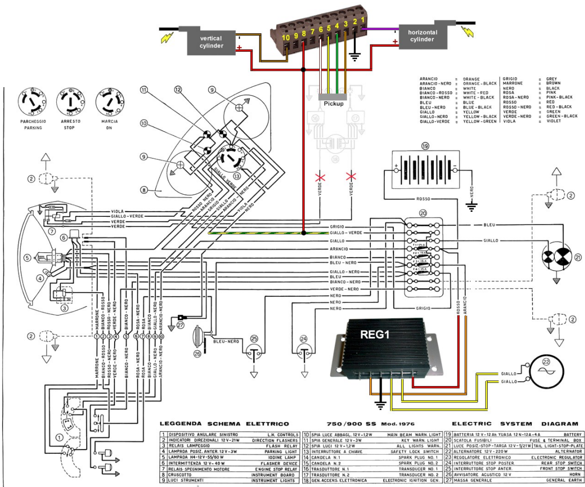
Complete wiring
