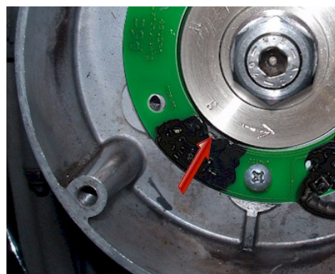
Figure 7.b The LED goes off when the piston is on TDC.
